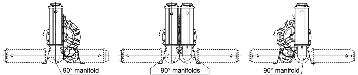
Fig.3 with two 90° manifolds
