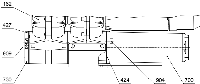
Fig.2 with 90° manifold
