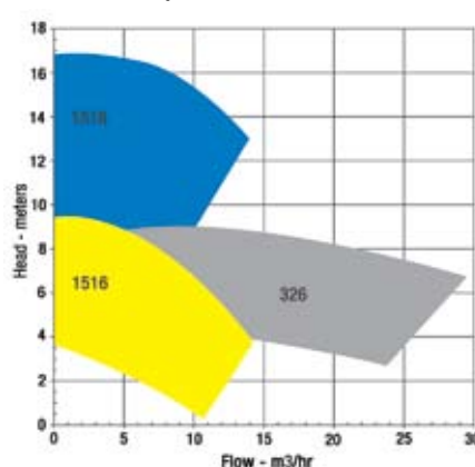
50 Hz, 1450 rpm
