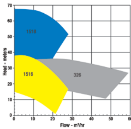
50 Hz, 1450 rpm
